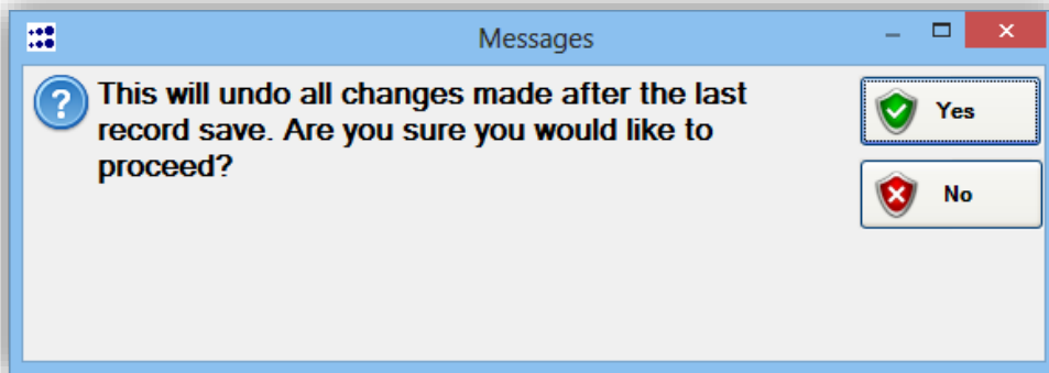
Figure 218 - Undo confirmation
