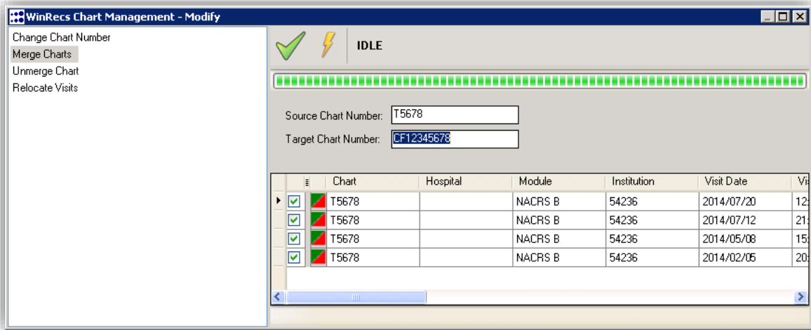
Figure 268 – Change Merge Example
