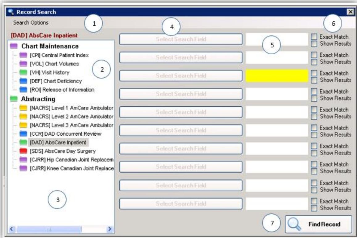
Figure 195 - Record Search Window
