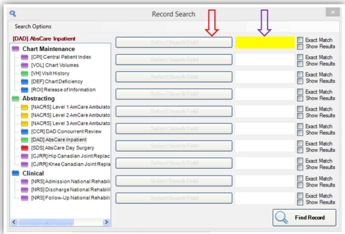
Figure 197 - Search Steps 2 & 3
