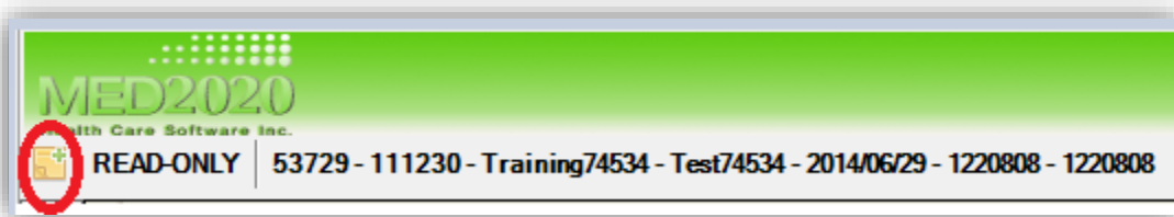
Figure 214 – Notes Icon
