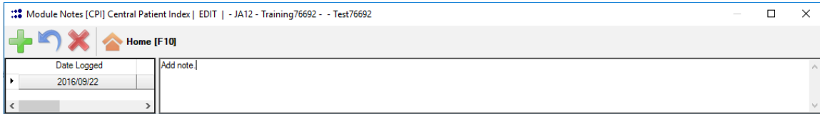
Figure 215 – Notes Window
