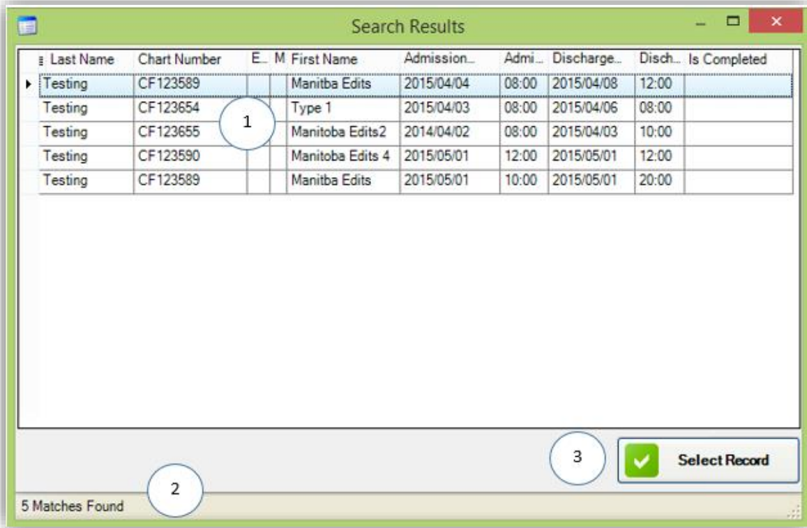
Figure 199 - Search Results
