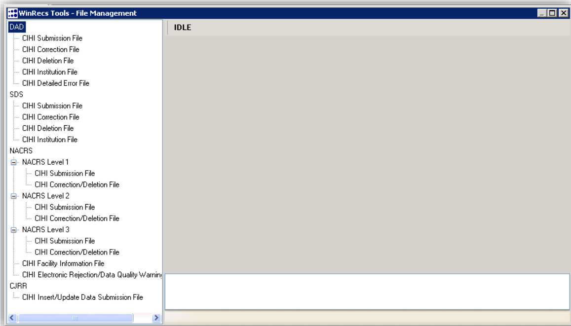
Figure 120 - File Management
