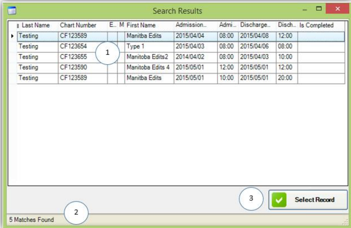
Figure 201 - Search Results
