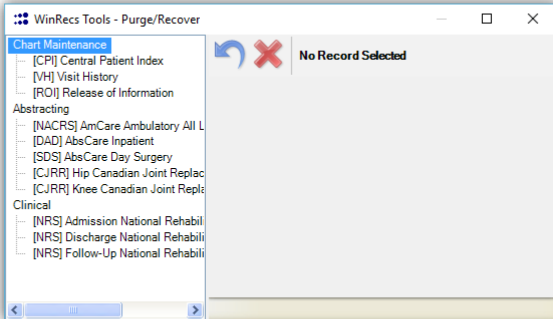
Figure 190 – Purge/Recover Screen
