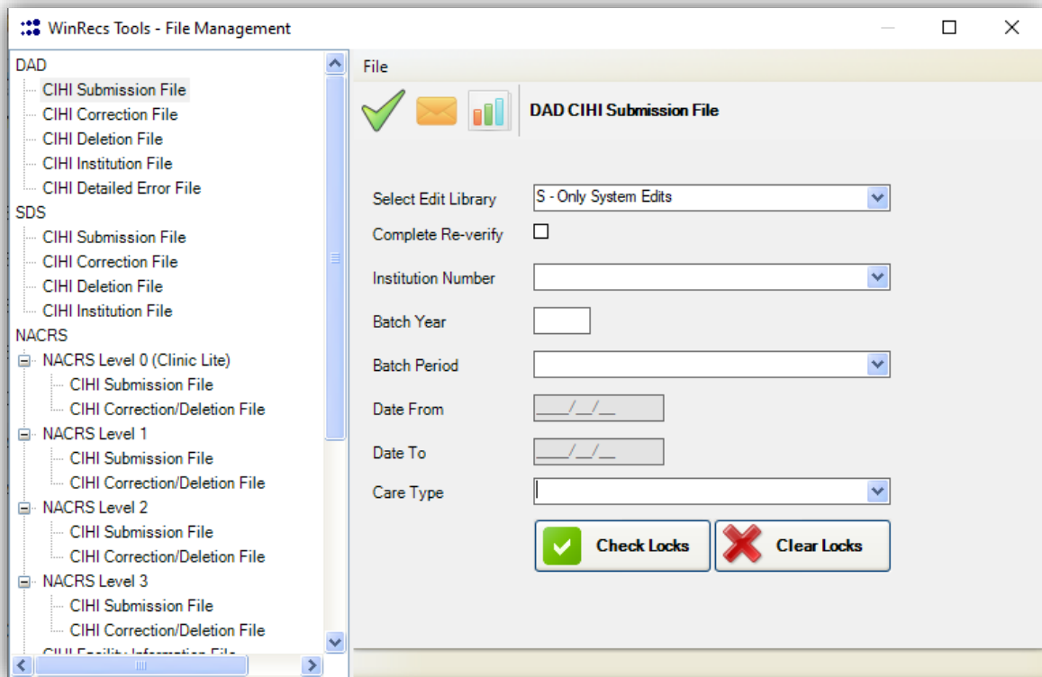
Figure 132 – File Management DAD/SDS/CJRR Submission File Screen
